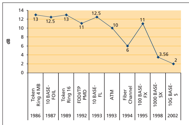
Figure 2: Fiber optic technologies vs. optical loss
